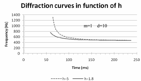
Fig.4 Variation of diffraction curves with height.
