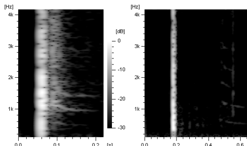
Fig.9 Chirp echo in function of the distance. Sonograms of an echo recorded at 5 and 50 meters respectively.
