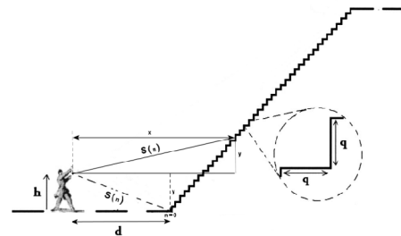
Fig.2 Pyramid's staircase and sound paths description.
